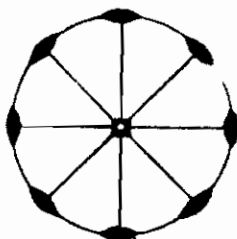
Tetragonal
