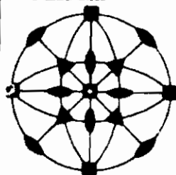
Cubic (Isometric)
